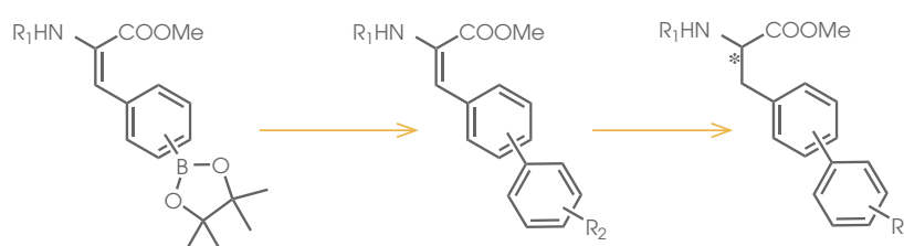
Suzuki coupling followed by asymmetric hydrogenation
